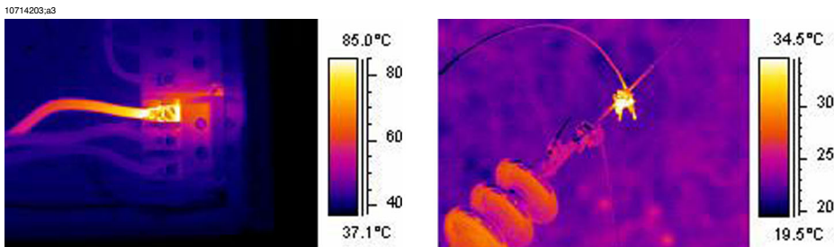
Figure 13.16 LEFT: An infrared image showing bad contact due to a loose bolt; RIGHT: A loose outdoor connection, exposed to the wind cooling effect.
